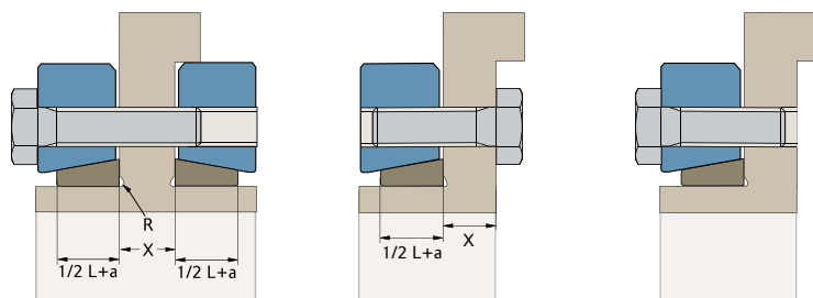
Split Shrink Disc
