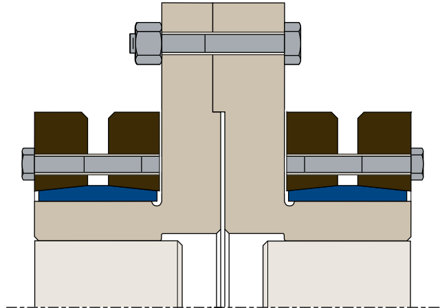
Flange-type Shrink Disc Coupling
