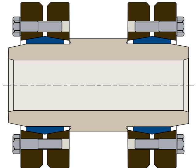
Sleeve-type Shrink Disc Coupling
