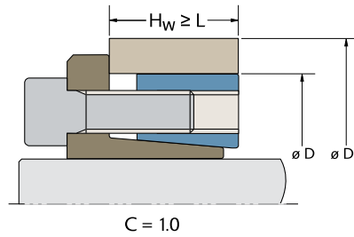
B-LOC® B109, B103, B106, B400, B800 & Trantorque®
