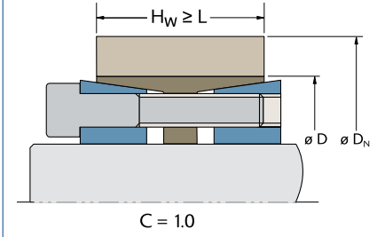
B-LOC® B112, B113, & B115
